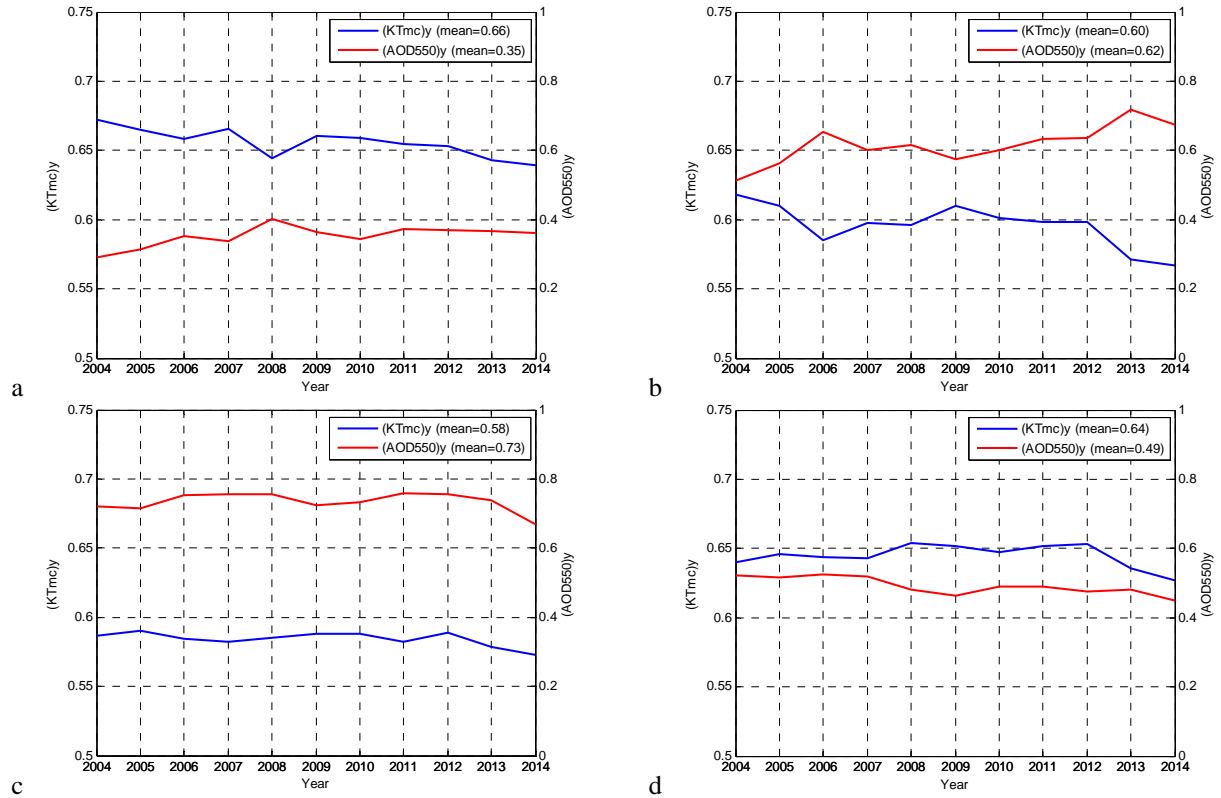
Fig. 2. (KT_{clear})_y from McClear, in blue, and (\tau_{550})_y from MACC, in red, from 2004 to 2014: (a) Harbin; (b) Beijing; (c) Wuhan; (d) Guangzhou
