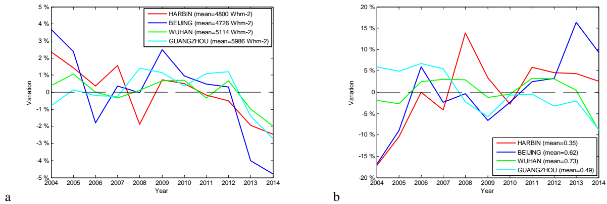
Fig. 1. (a) Variation of a) (G_{clear})_y and b) (\tau_{550})_y with respect to their long term average from 2004 to 2014.
